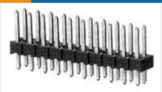
TE Part # 5-102617-8 20 MODII HDR DRRA SHRD LF
