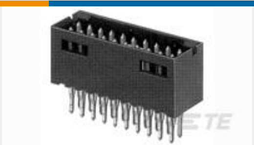
TE Part # 6-146261-0 20 MODII HDR DRST B/A .100CL LF
